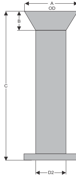
Bellmouth
