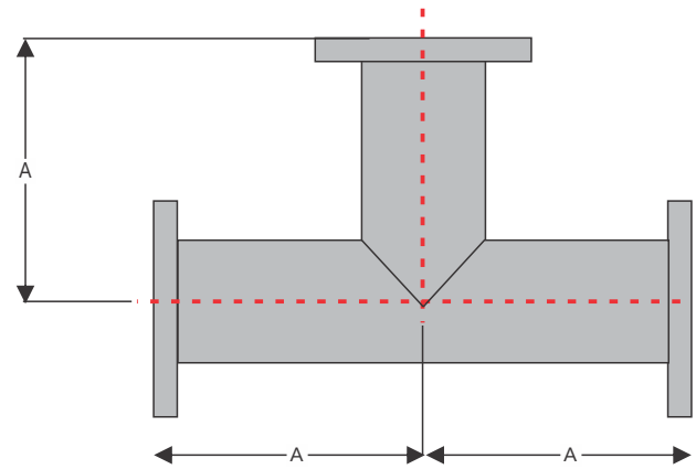
Flanged Ends
