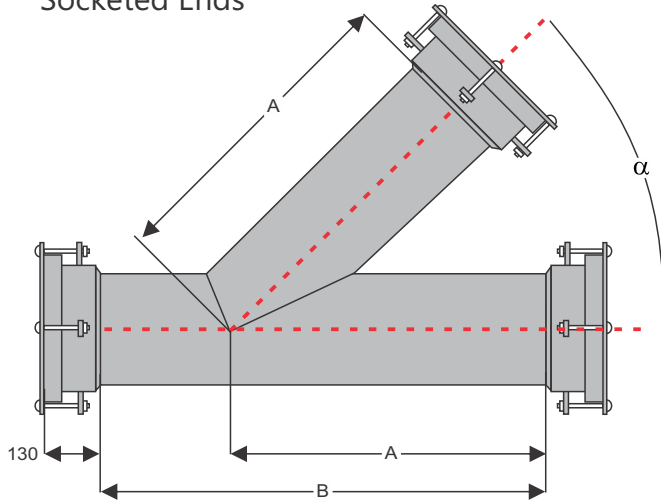
Socketed Ends
